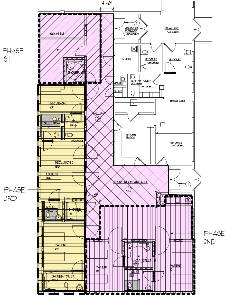
① PHASING PLAN T2.0 SCALE: 1/8" = 1'-0"
